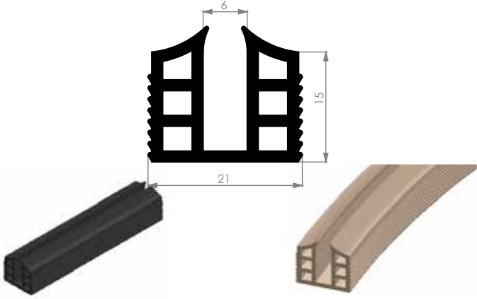
ALM. GENEL FİTİLLER 08-34
