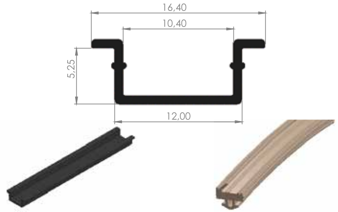
ALM. GENEL FİTİLLER 08-29
