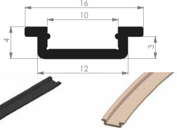
ALM. GENEL FİTİLLER 08-35
