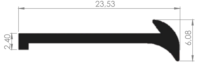
ALM. GENEL FİTİLLER 08-25
