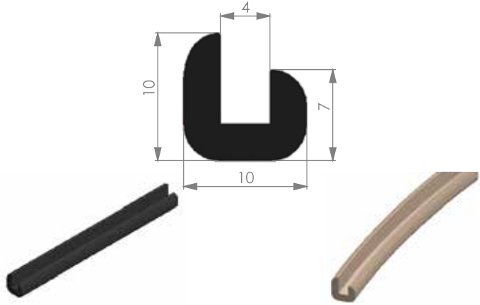
ALM. GENEL FİTİLLER 08-36
