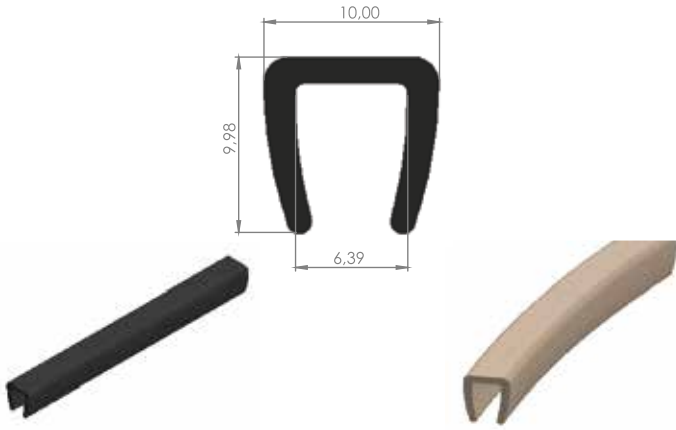
ALM. GENEL FİTİLLER 08-08
