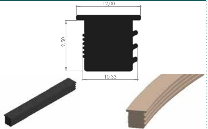
ALM. GENEL FİTİLLER 08-19
