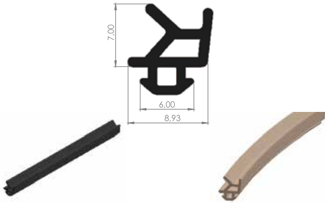
ALM. GENEL FİTİLLER 08-28
