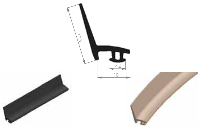
ALM. GENEL FİTİLLER 08-32
