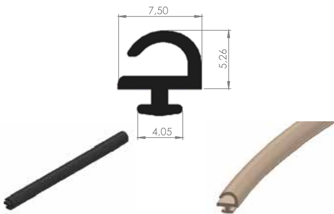
ALM. GENEL FİTİLLER 08-17
