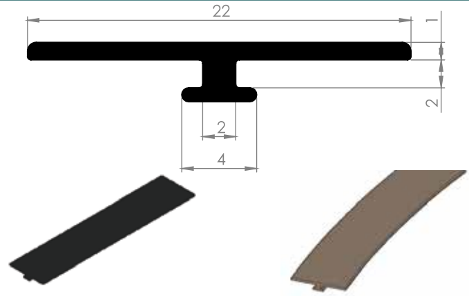
ALM. GENEL FİTİLLER 08-31
