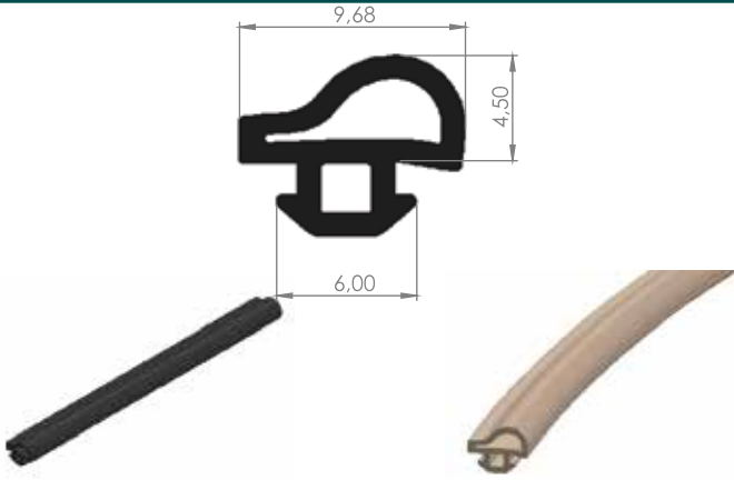
ALM. GENEL FİTİLLER 08-18
