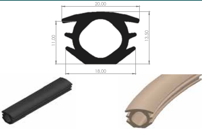
ALM. GENEL FİTİLLER 08-39 DERZ FİTİLİ
