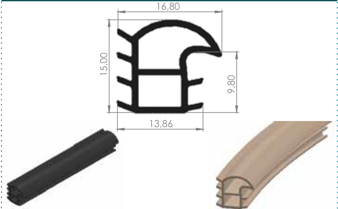
ALM. GENEL FİTİLLER 08-06
