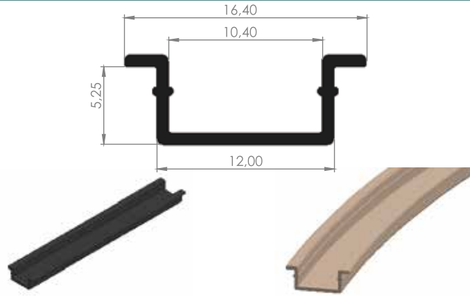
ALM. GENEL FİTİLLER 08-30
