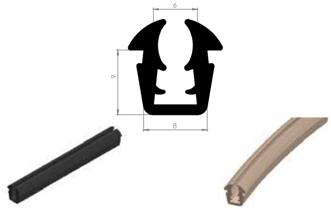
ALM. GENEL FİTİLLER 08-33
