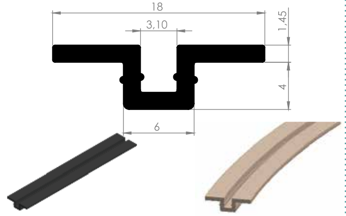
ALM. GENEL FİTİLLER 08-09
