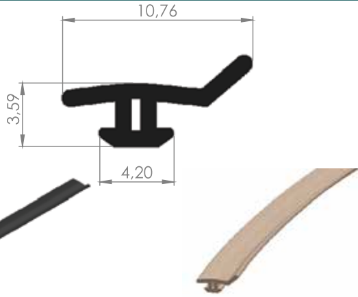
ALM. GENEL FİTİLLER 08-15
