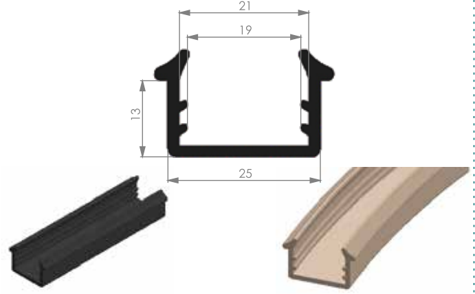
ALM. GENEL FİTİLLER 08-37
